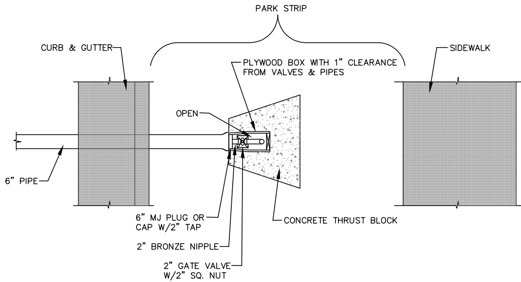
THRUST BLOCK DETAIL PLAN VIEW
